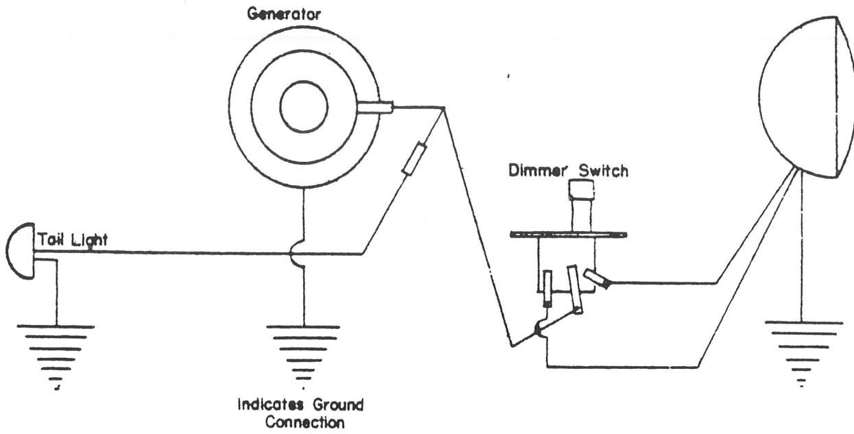
FIGURE 39 WIRING DIAGRAM FOR 52-53A-54
