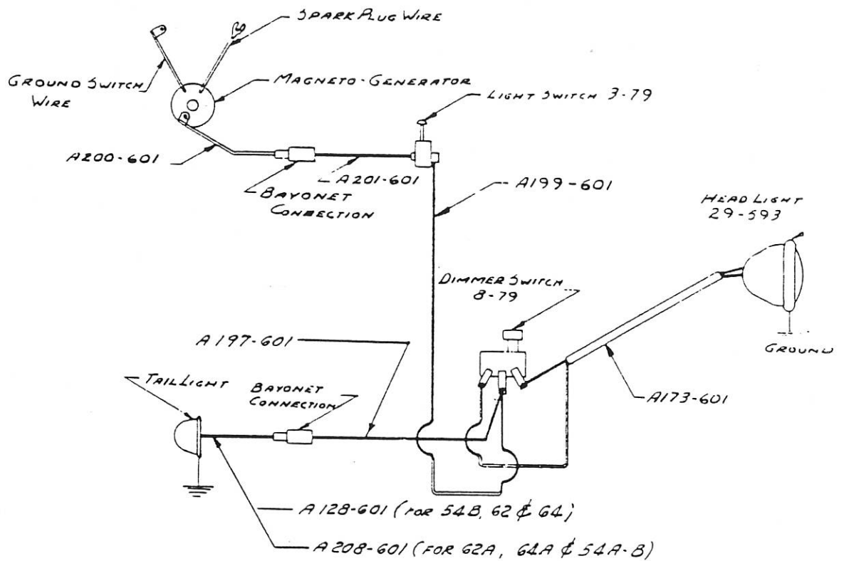
Figure 35: Wiring Diagram Models 62 - 64
