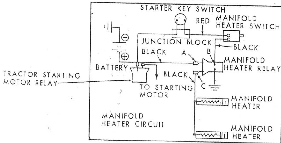
CIRCUIT WIRING DIAGRAM 12-VOLT SYSTEM
