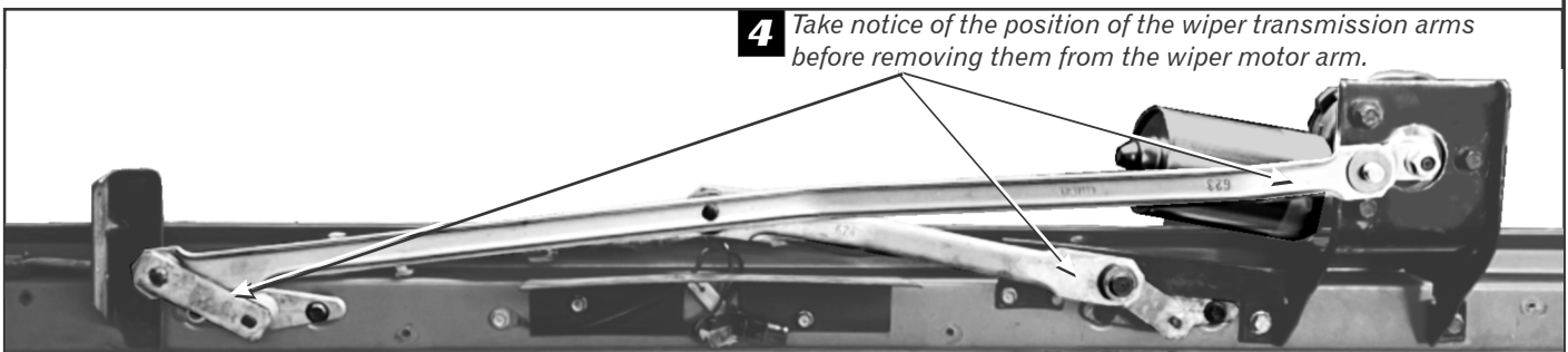
View of wiper motor mechanism installed on windshield frame
