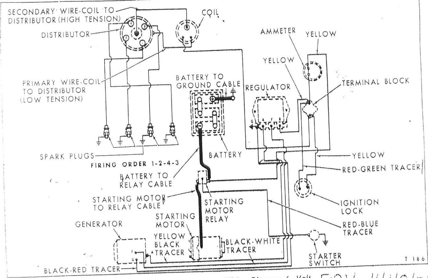
Wiring Diagram 6-Volt FDN-14401-B
